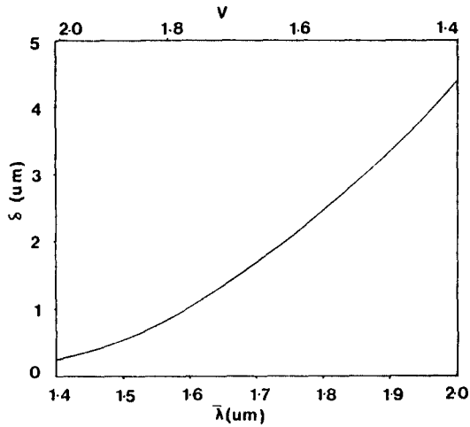
Fig.10 Optimum-core spacings v · s various center-wavelengths.
