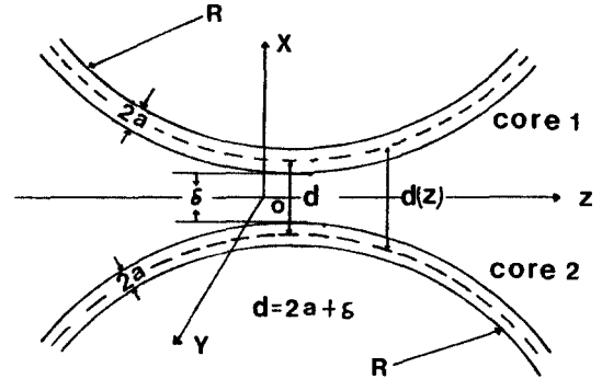
Fig.1 Lateral section of the optical coupler.
