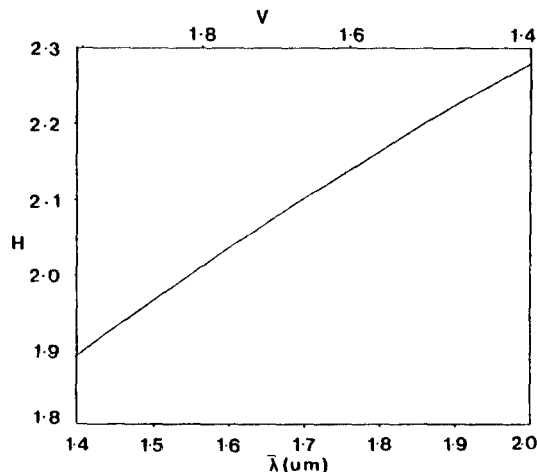
Fig.9 H value v · s various center-wavelengths
