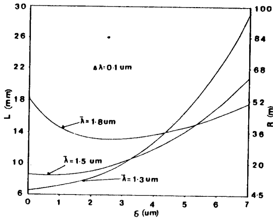
Fig.6 L and R v · s various core-spacings.
