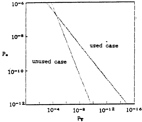
P_t : BER of transmission line P_o : Total BER at optical terminal system
