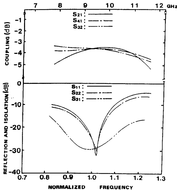
Fig. 6. Measured Response Curves for the 7\lambda/6 ring Directional Coupler
