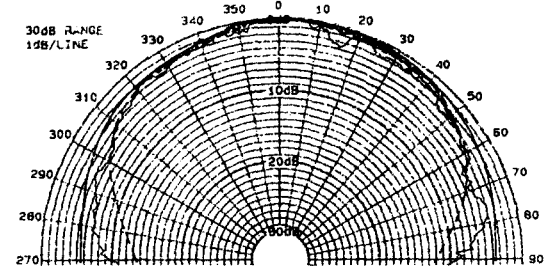
(b) radiation pattern of E_\phi .
