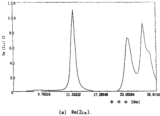
(a) Re(Z_{in}) .
