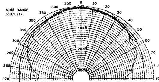
(b) radiation pattern of E_{\theta} .
