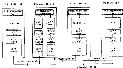
Fig. 4. D and G-interfaces and Clearing House in an integrated network
