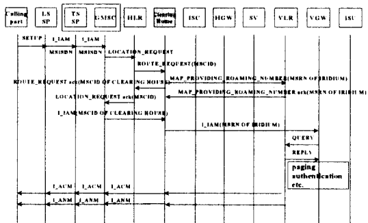
Fig. 7. Terminating call setup procedure for the roaming subscriber in the IRIDIUM system
