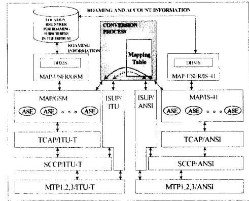
Fig. 3. Architecture of Clearing House
