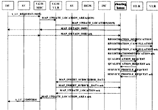
Fig. 6. Location registration signaling message flow (Move from CDMA system to IRIDIUM)
