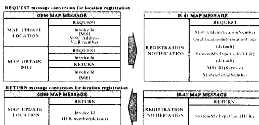
Fig. 5. Message conversion for location registration between IRIDIUM and CDMA systems
