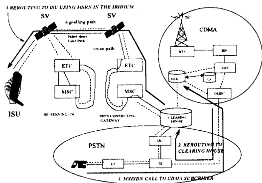
Fig. 8. Routing to dual-mode-terminal roaming in the IRIDIUM system
