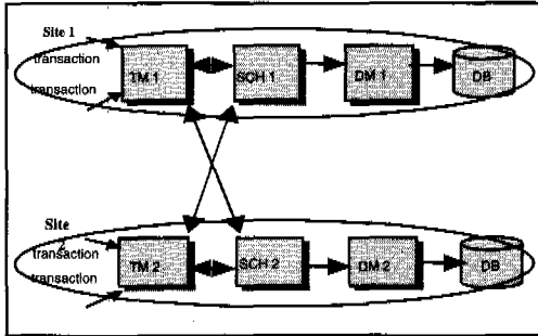
Fig. 3 2DL Transaction Processing Model
