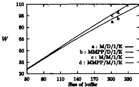
Fig. 12 Mean delay vs. buffer size ( r_1=0.01 , r_2=0.05 , \lambda_1=1.0 , \lambda_2=0.99 , h=1.0 )
