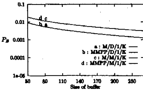
Fig. 11 Loss probability vs. buffer size ( r_1=0.01 , r_2=0.05 , \lambda_1=1.0 , \lambda_2=0.99 , h=1.0 )
