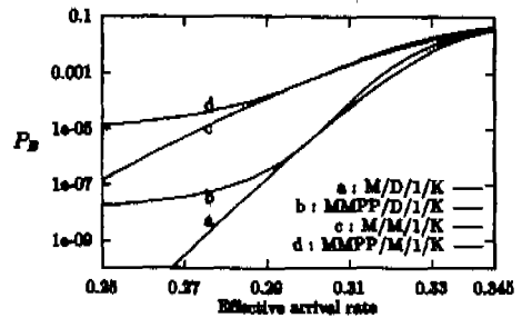
Fig. 5 Loss prob. vs. effective arrival rate ( r_1=0.01, r_2=0.05, \lambda_1=0.3, K=51, h=3.0 )
