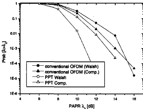
Fig. 10 Probability that an OFDM-CDMA symbol exceeds specific PAPR \lambda_0 with 16 active users
