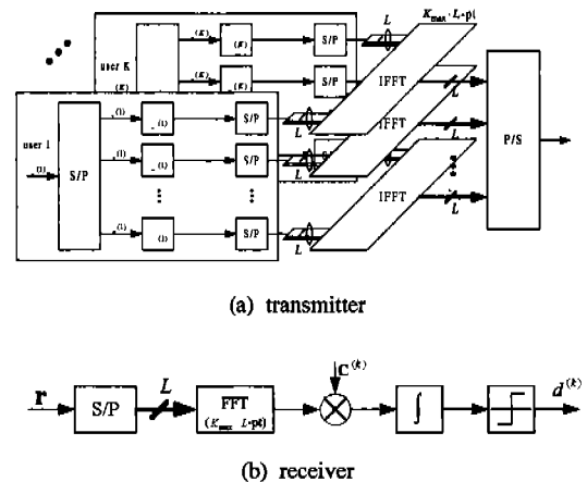
Fig. 2 Partial Parallel Transformed OFDM-CDMA system
