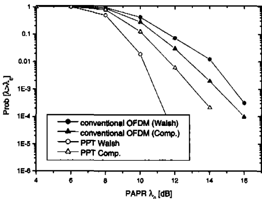
Fig. 9 Probability that an OFDM-CDMA symbol exceeds specific PAPR \lambda_0 with 14 active users
