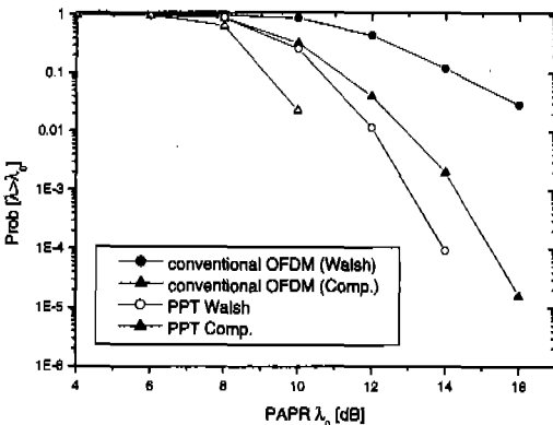
Fig. 4 Probability that an OFDM-CDMA symbol exceeds specific PAPR \lambda_0 with 4 active users
