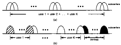
Fig. 1 Input Data Structures of IFFT in (a) conventional OFDM-CDMA and (b) PPT-OFDM-CDMA System
