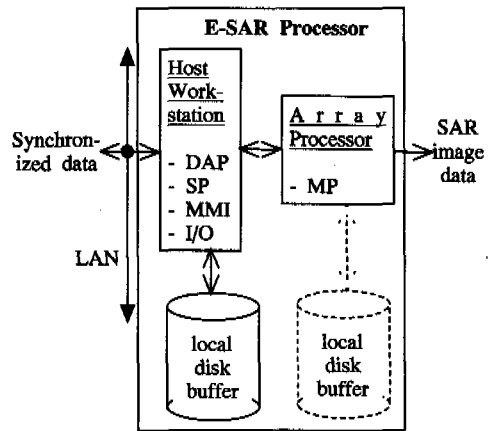
Fig. 3 Top level HW mapping of the E-SAR processor
