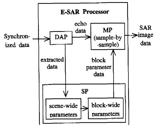
Fig. 2 Top level SW mapping of the E-SAR processor
