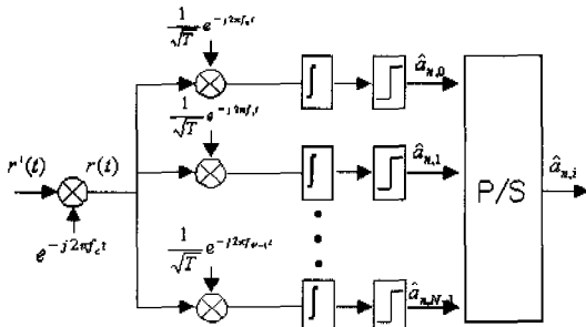
Fig. 6 The structure of OFDM receiver.
