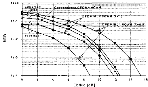
Fig. 10 BER performance of OFDM/HL-16QAM system in AWGN channel.
