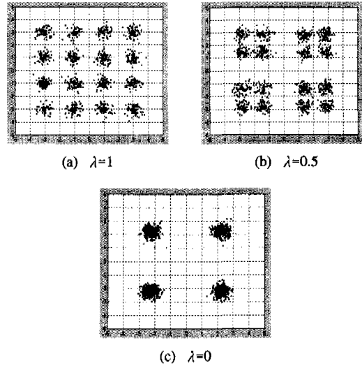
Fig. 9 Constellation for the OFDM/HL-16QAM system in two ray multipath channel ( E_b/N_0 = 40 dB).
