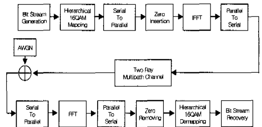
Fig. 7 Simulation block diagram of OFDM/HL-16QAM system.
