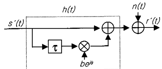
Fig. 5 Two ray multipath channel model.
