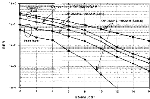
Fig. 12 BER performance of OFDM/HL-16QAM system in two ray multipath fading channel.
