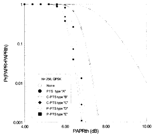
(b) N = 256
