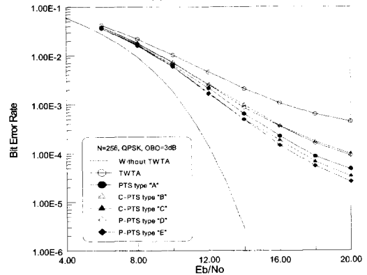
(b) N = 256
