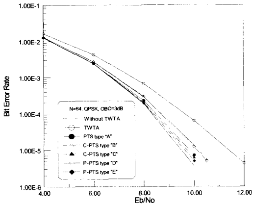
(a) N = 64
