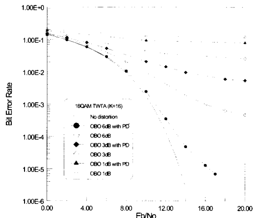
(b) 16QAM (K =16)
