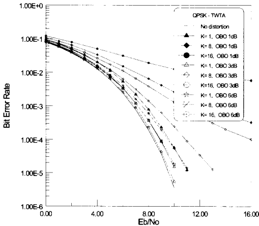
(a) QPSK
