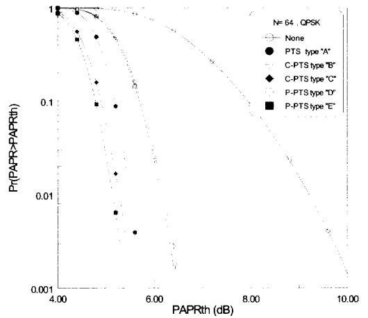
(a) N = 64
