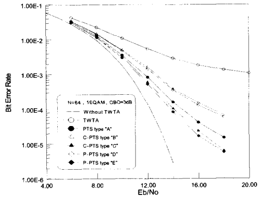
(a) N = 64
