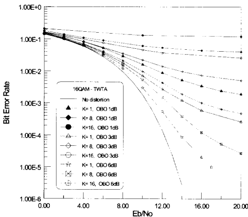
(b) 16QAM
