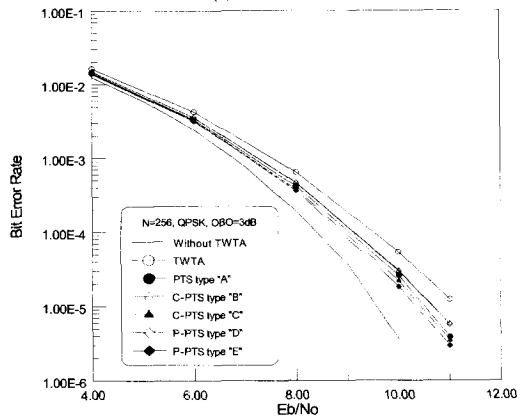
(b) N = 256
