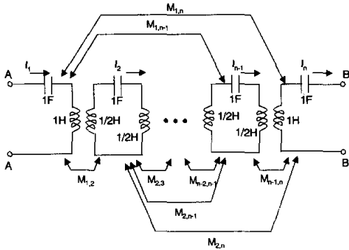
Fig. 3. Equivalent circuit with LC elements for n-pole synchronously tuned filter.
