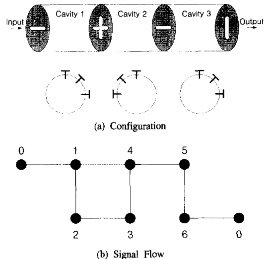
Fig. 6. 6-Pole dual-mode filter with cross coupling at M14.
