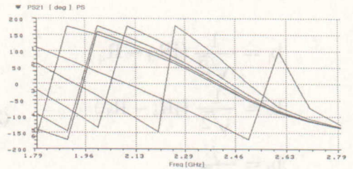
그림 5. Simulation results of phase shift versus input DC voltage with the frequency range of 1.79-2.79GHz.
