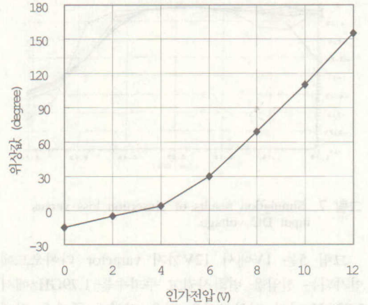
그림 11. Measured phase shift as a function of the DC bias versus variable input DC voltage
