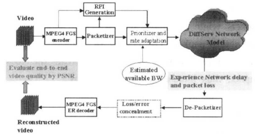
Fig. 4 The diagram of proposed experiment setup.
