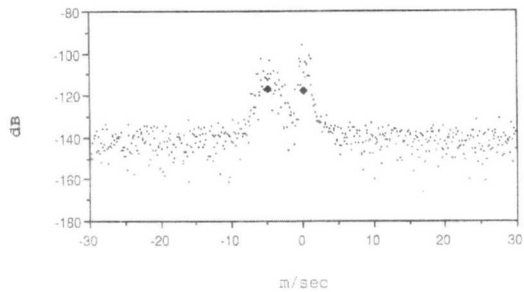
Fig. 2. Mode estimates shown in the simulated weather spectrum of range cell 29
