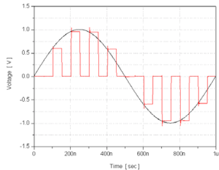
(b) SHA2
