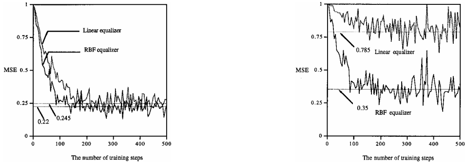
(a) desired symbol, a_{k-d} = a_{k-1} (b) desired symbol, a_{k-d} = a_k (no channel delay) Fig. 2. Comparison of MSE convergence H(z) = 0.5 + z^{-1} , \sigma_n^2 = 0.1
