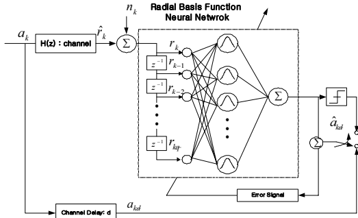
Fig. 1. The block diagram of RBF equalizer
