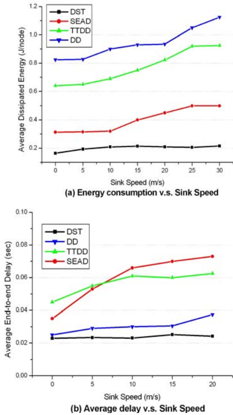
Fig.10. Impact of sink's mobility
