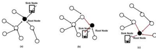
Fig.2. Description of basic DST operation
