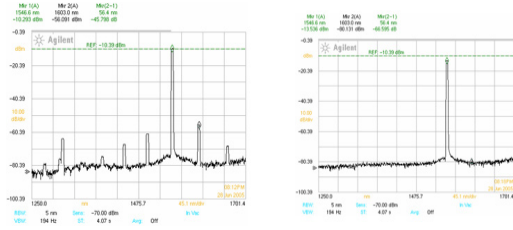
(a) RN (상향) (b) OLT(상향)
