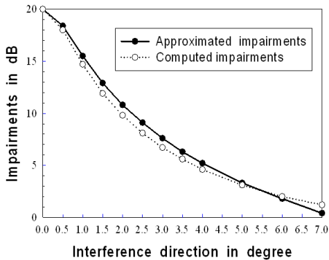
Fig. 1 Approximated and computed impairments as a function of direction, \gamma_d = 20 dB, \gamma_i = 10 dB, N = 10 , \theta_d = 0^\circ , d = \lambda/2
