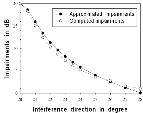
Fig. 2. Approximated and computed impairments as a function of direction, \gamma_d = 20 dB, \gamma_i = 10 dB, N = 10 , \theta_d = 20^\circ , d = \lambda/2
