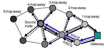
(a) AODV
