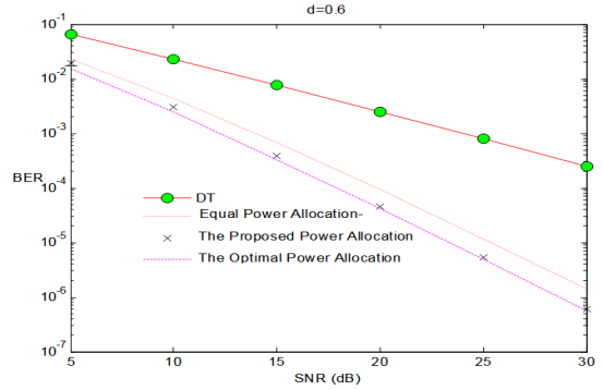
Fig. 7. BER performance with energy allocation strategies with d=0.6
