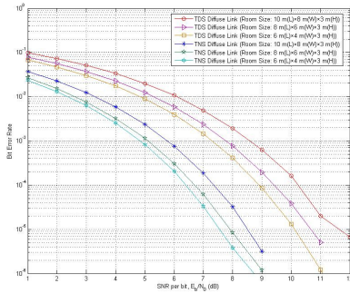
Fig. 17. Simulation results of BER based on different room size
