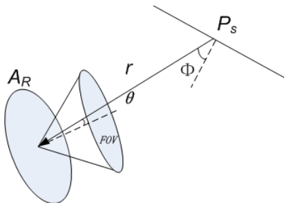
Fig. 4. Receiver model
