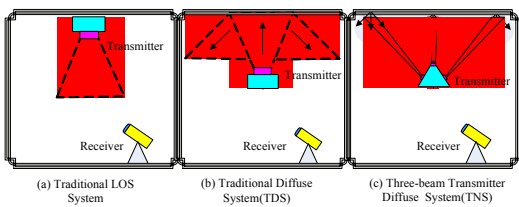
Fig. 2. Wireless optical communication channel configuration
