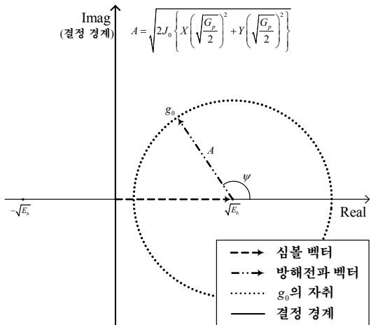
(b) \frac{E_b}{J_0} > 2 \left\{ X \left( \sqrt{\frac{G_p}{2}} \right)^2 + Y \left( \sqrt{\frac{G_p}{2}} \right)^2 \right\} 인 경우
