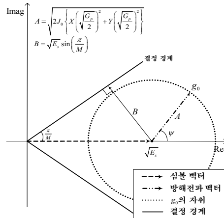
(c) \frac{2}{k} \frac{\left\{ X \left( \sqrt{\frac{G_p}{2}} \right)^2 + Y \left( \sqrt{\frac{G_p}{2}} \right)^2 \right\}}{\sin^2(\pi/M)} < \frac{E_b}{J_0} 인 경우
