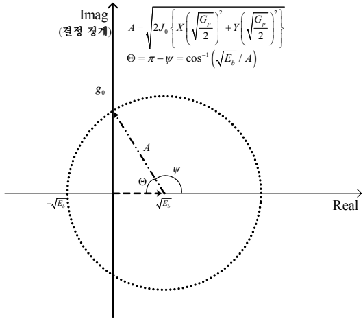
(a) \frac{E_b}{J_0} \leq 2 \left\{ X \left( \sqrt{\frac{G_p}{2}} \right)^2 + Y \left( \sqrt{\frac{G_p}{2}} \right)^2 \right\} 인 경우
