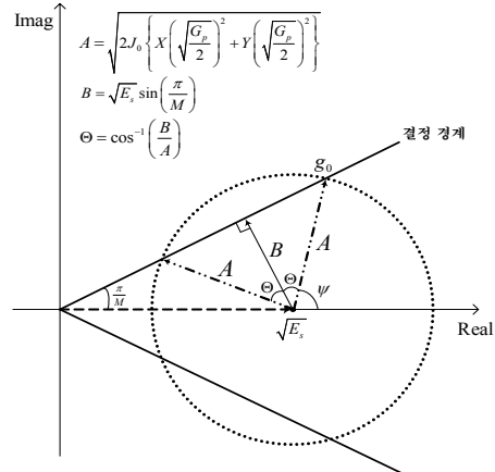
(b) \frac{2}{k} \left\{ X \left( \sqrt{\frac{G_p}{2}} \right)^2 + Y \left( \sqrt{\frac{G_p}{2}} \right)^2 \right\} < \frac{E_b}{J_0} \leq \frac{2}{k} \frac{\left\{ X \left( \sqrt{\frac{G_p}{2}} \right)^2 + Y \left( \sqrt{\frac{G_p}{2}} \right)^2 \right\}}{\sin^2(\pi/M)} 인 경우
