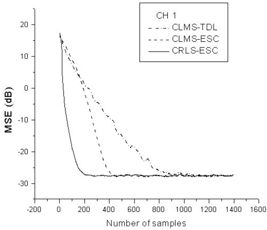
Fig. 2. MSE convergence performance in CH 1.
