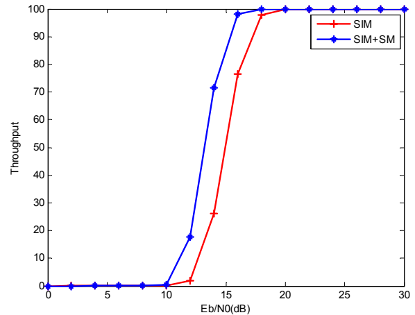
Fig. 8. Throughput versus SNR for propose SIM+SM and SIM scheme when spectral efficiency of 2bits/s/Hz
