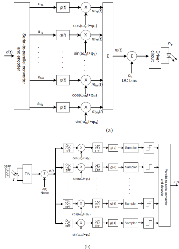
Fig. 1. Block diagram of SIM-FSO. (a) Transmitter and (b) receiver.
