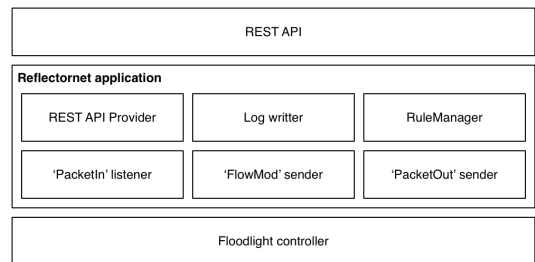
Fig. 7. Reflector network architecture
