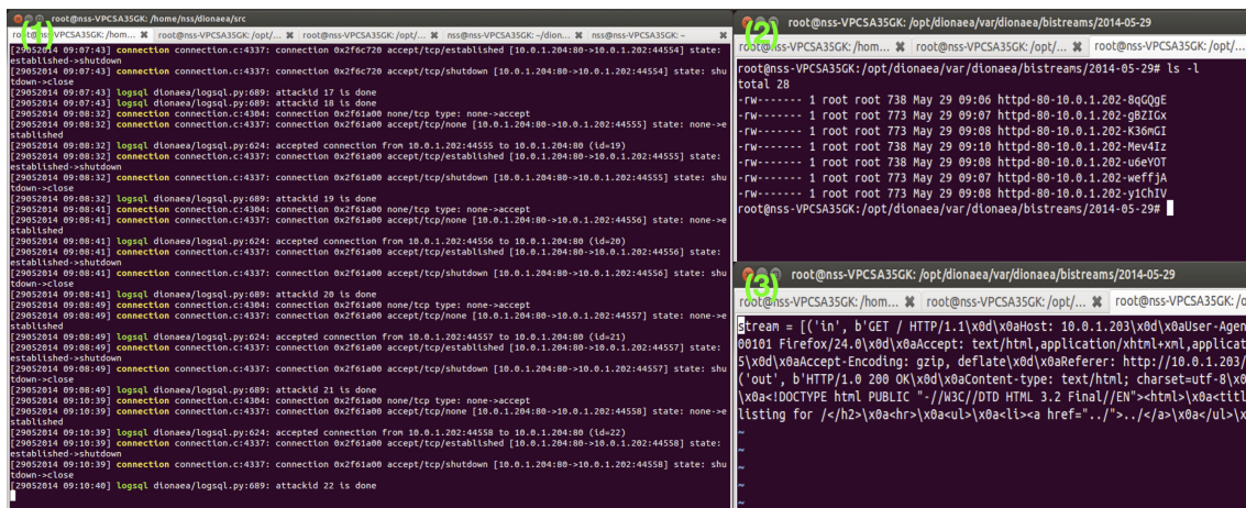
Fig. 10. honeypot behavior (1) Real time log (2) Collected list (3) Collected data
