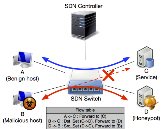
Fig. 6. SDN based Reflector network. Both hosts want to connect with the service. However the malicious host can't connect with the service, instead connect with the honeytrap.
