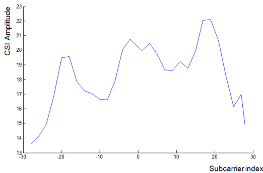
(a) Frequency Domain CSI
