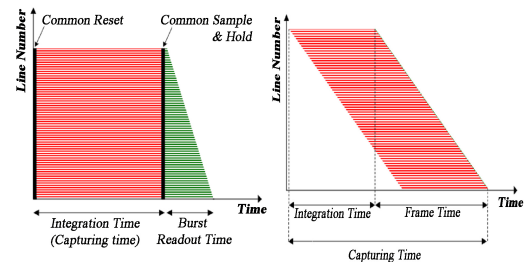
Fig. 3. Rolling shutter and global shutter operation
