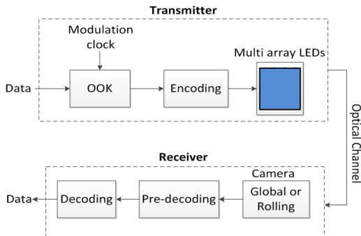
Fig. 2. Camcom transmitter and receiver structure
